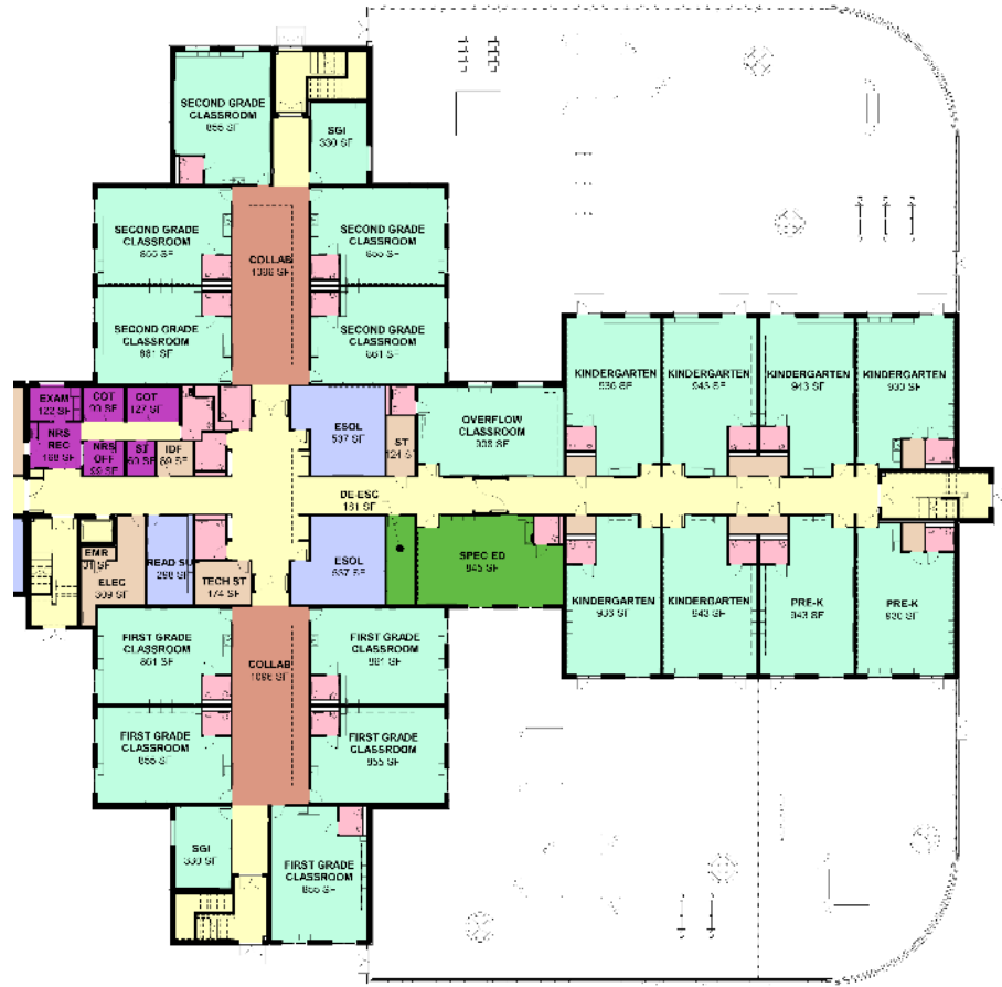
Partial First Floor Plan – 2-story
